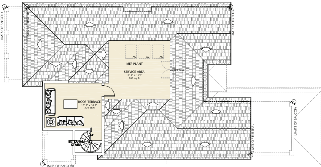
Roof Top
